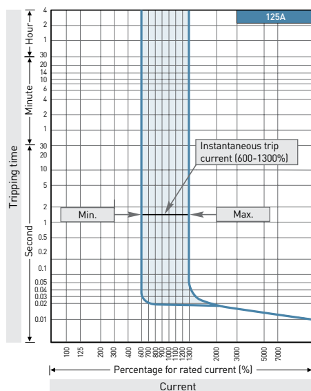
Tripping curves
