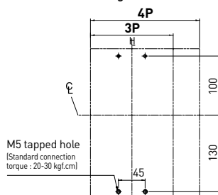
[Drilling holes for mounting]
