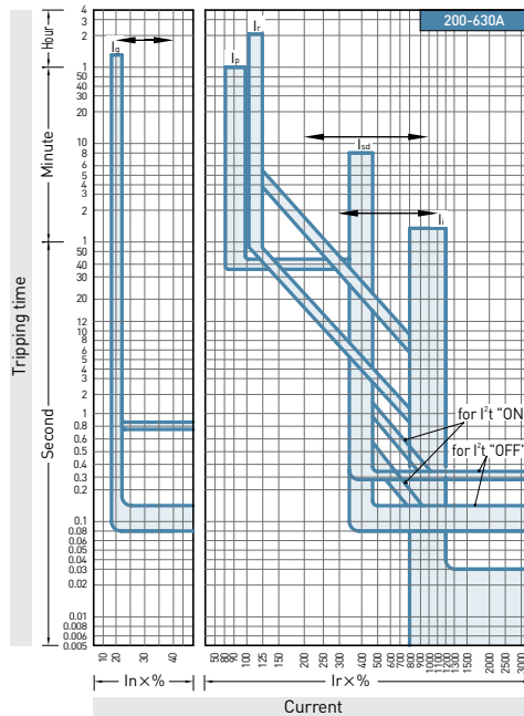
Tripping curves
