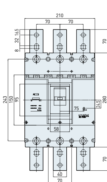
[Terminal part]
