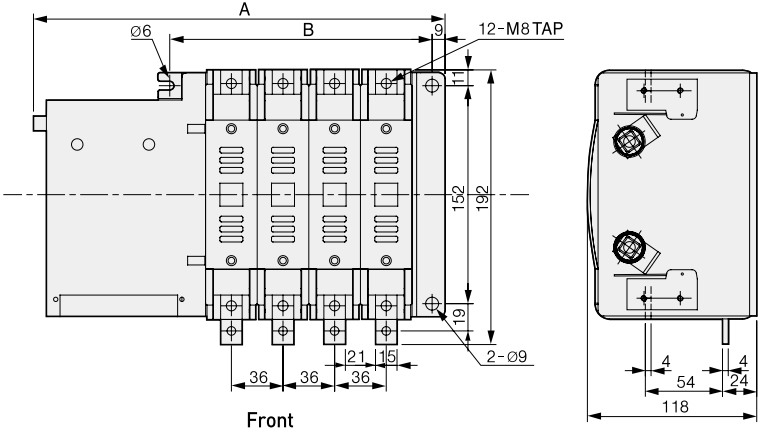
WN B-Type100A~200A
