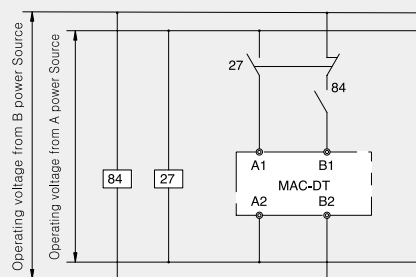
Operating Circuit 1
