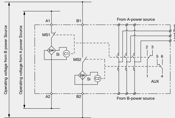
Control Circuit Diagram
