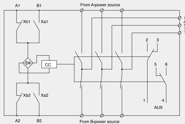
Internal Circuit
