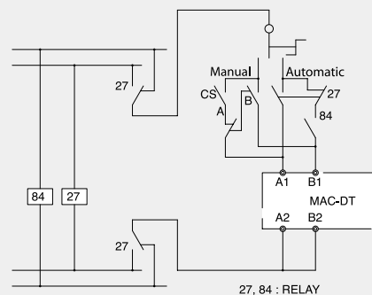
Operating Circuit 2
