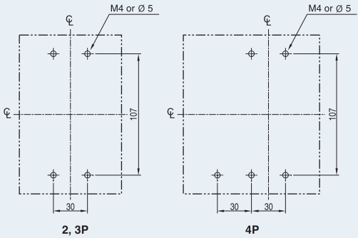
Panel drilling
