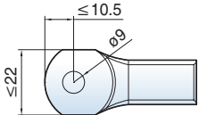
Terminal dimensions
