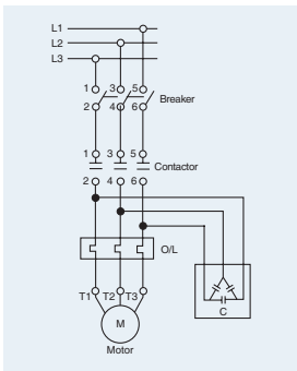
Capacitor circuit
