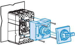
Extended rotary handles
