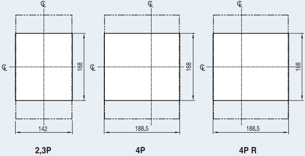
Front panel cutting
