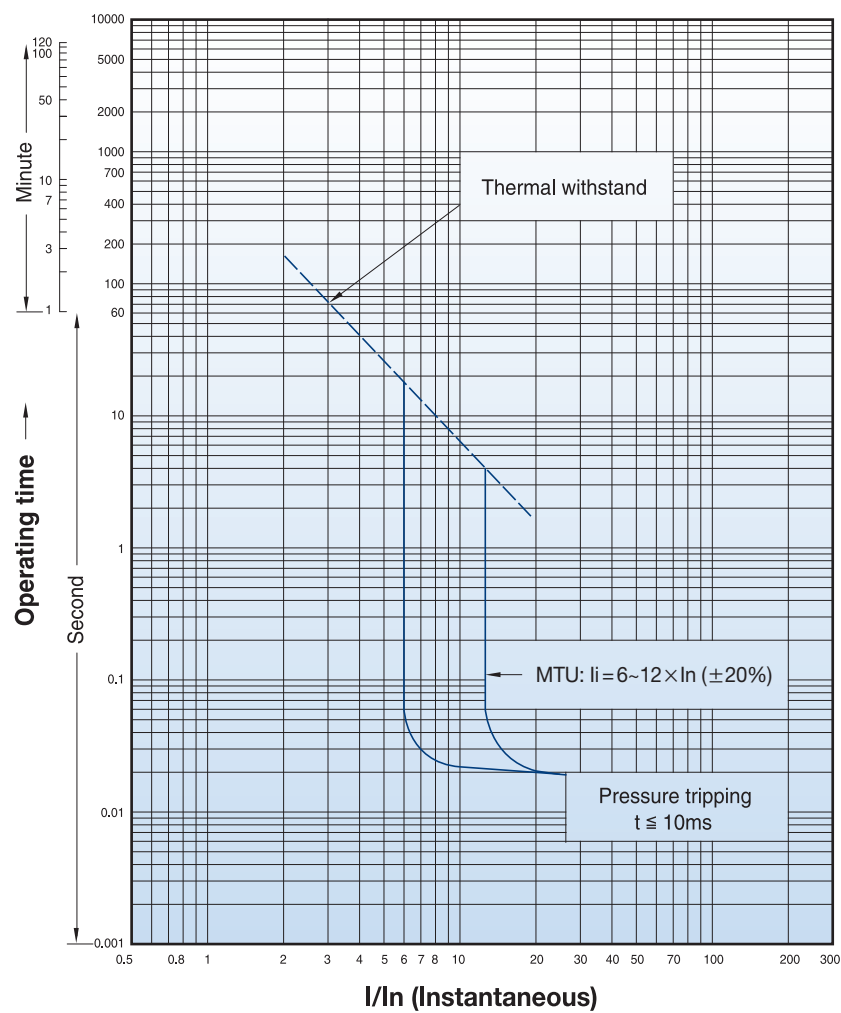
Magnetic trip units(MTU)
