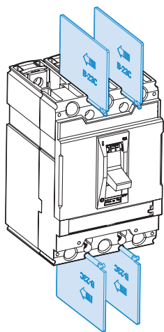
Insulation barriers
